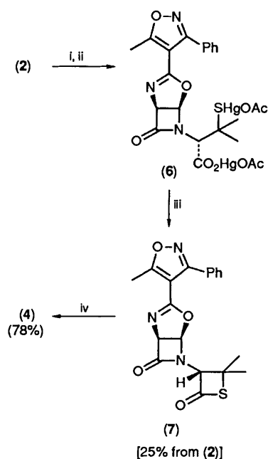
Scheme 2. Reagents and conditions: i, Hg(OAc) 2 , HOAc; ii, lyophilisation; iii, ClCO 2 Me (4 mol equiv.), pyridine; iv, BF 3 ·Et 2 O, CH 2 Cl 2 .
